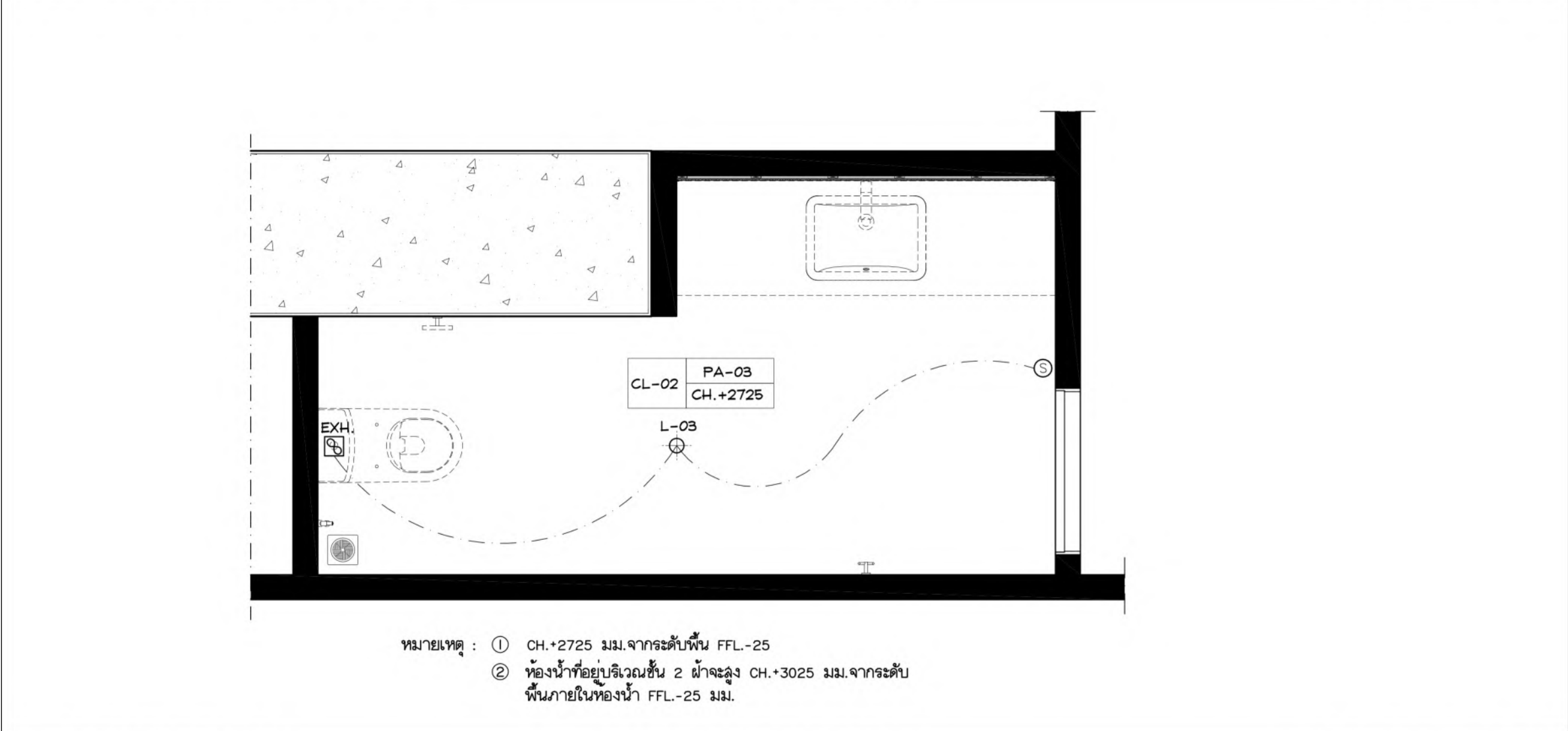
LIGHTING PLAN ( TYPE T-4 ) SCALE 1 : 25
