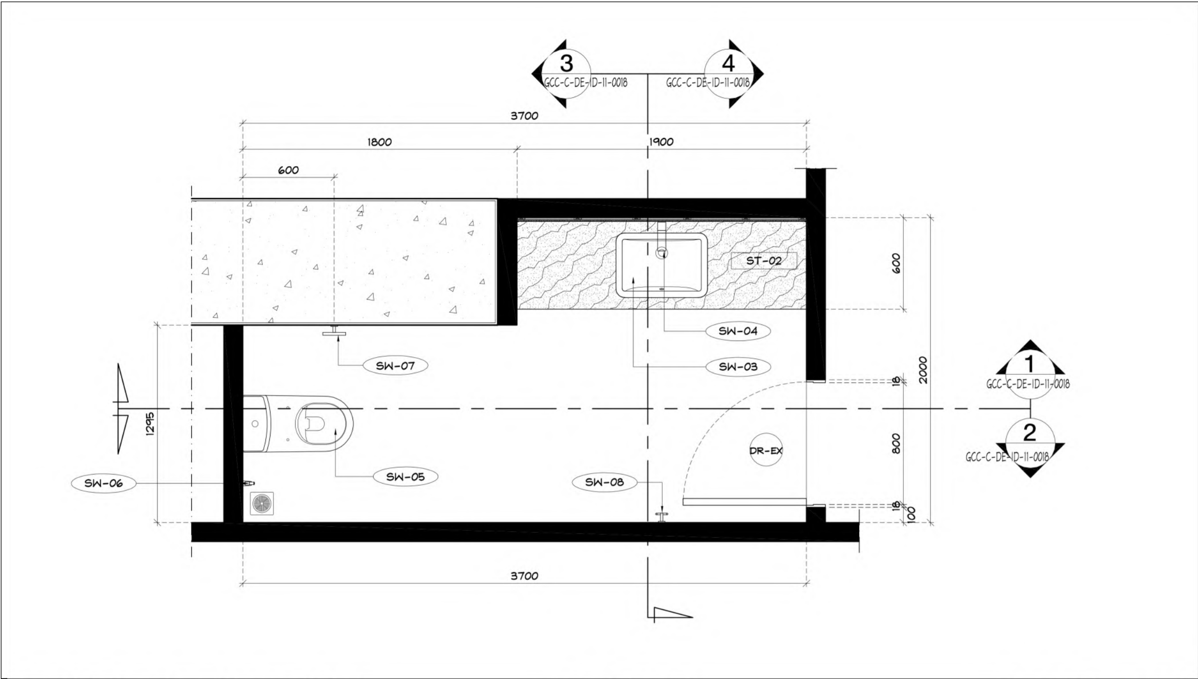
FURNITURE LAYOUT PLAN ( TYPE T-4 ) SCALE 1 : 25
