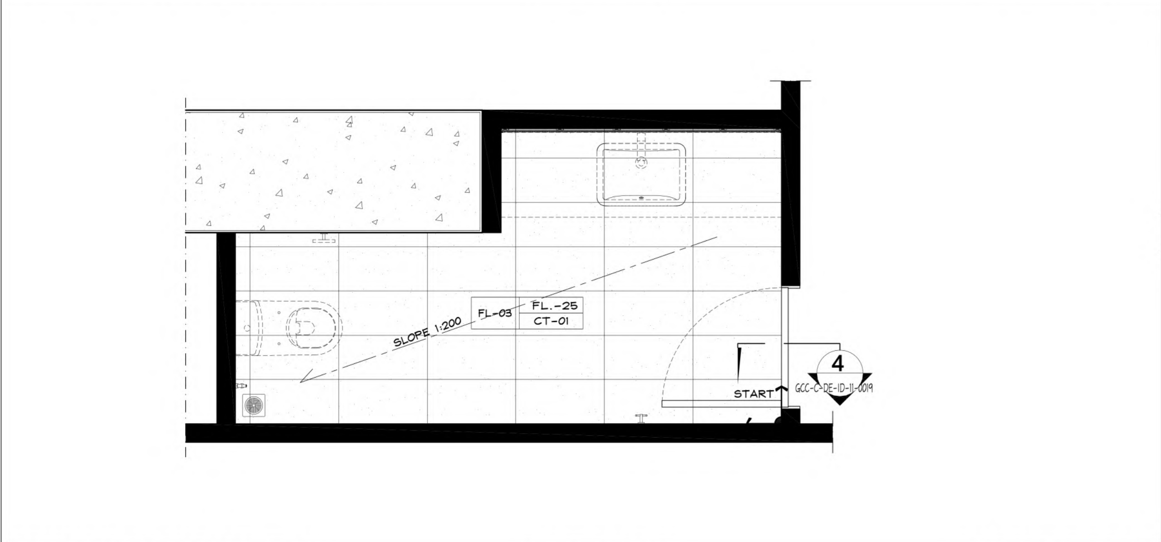
FLOOR FINISHING PLAN ( TYPE T-4 ) SCALE 1 : 25
